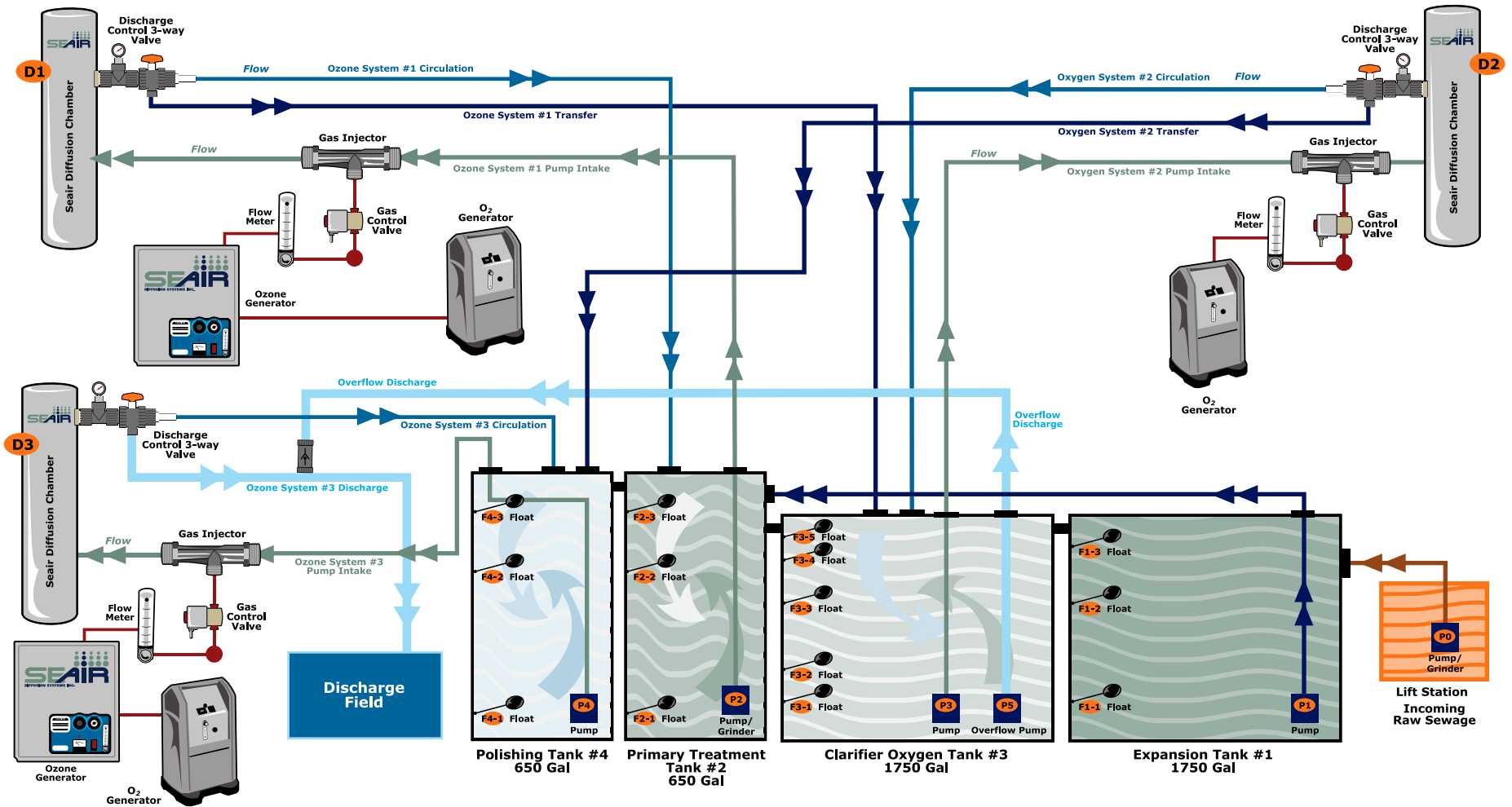
Seair Septic System PWW-40
